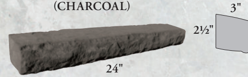
CHISELED STONE SILL (CHARCOAL)
